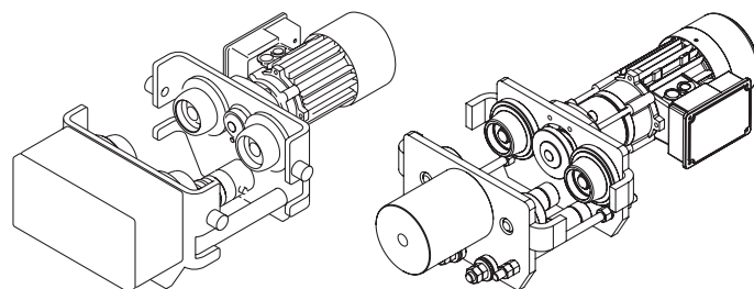
KM Monorail Trolley
